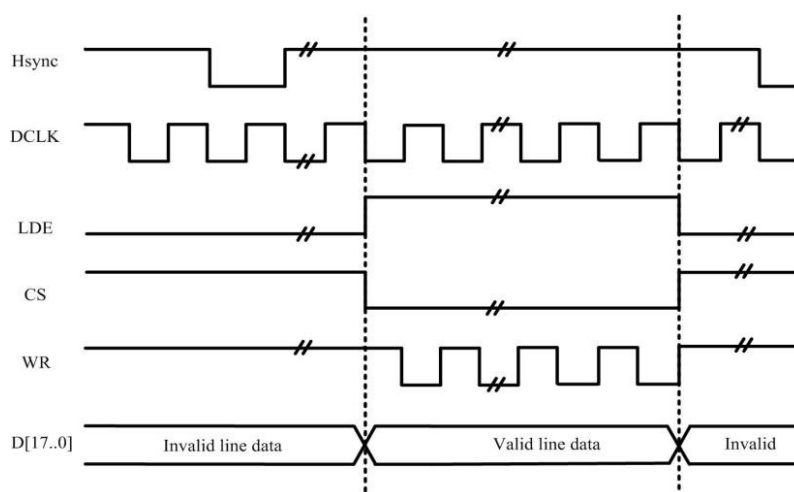
Figure 7-7. Lcd_CPUI/F Timing
