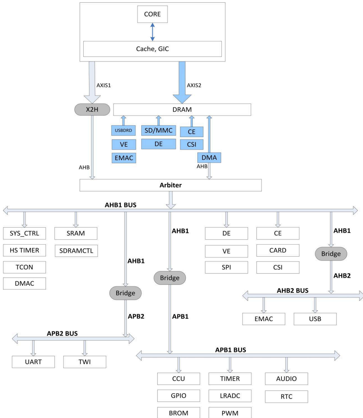
Figure 4-2. System Bus Tree
